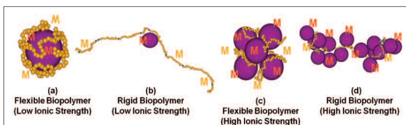
Fig. 3. Computer modelling of biopolymer-inorganic colloid (purple spheres) aggregate formation processes (Ulrich et al. 2006a). According to the pH (controlling the biopolymer ionization degree but also surface charge density of the inorganic colloid and TM binding affinity), conformation of ionisable biopolymers (yellow chain) may change drastically with charge density. Ionic strength is also expected to control the importance of the electrostatic interactions (biopolymer monomer-monomer, inorganic colloids-biopolymers, TM-biopolymer (M) and TM-inorganic (M) adsorption processes). Biopolymer flexibility (intrinsic and electrostatic) is also expected to control the final structures of the TM-inorganic and biopolymer aggregates hence resulting in the formation of very heterogeneous structures from dense and collapsed conformations to more extended structures (important effect on the settling velocities). At low ionic strength the flexible biopolymer is found here to stabilize the inorganic colloid mainly by steric and electrostatic effects whereas the rigid biopolymer to promote bridging processes between inorganic colloids. At high ionic strength the biopolymer is expected to promote the aggregate formation in the two cases.
