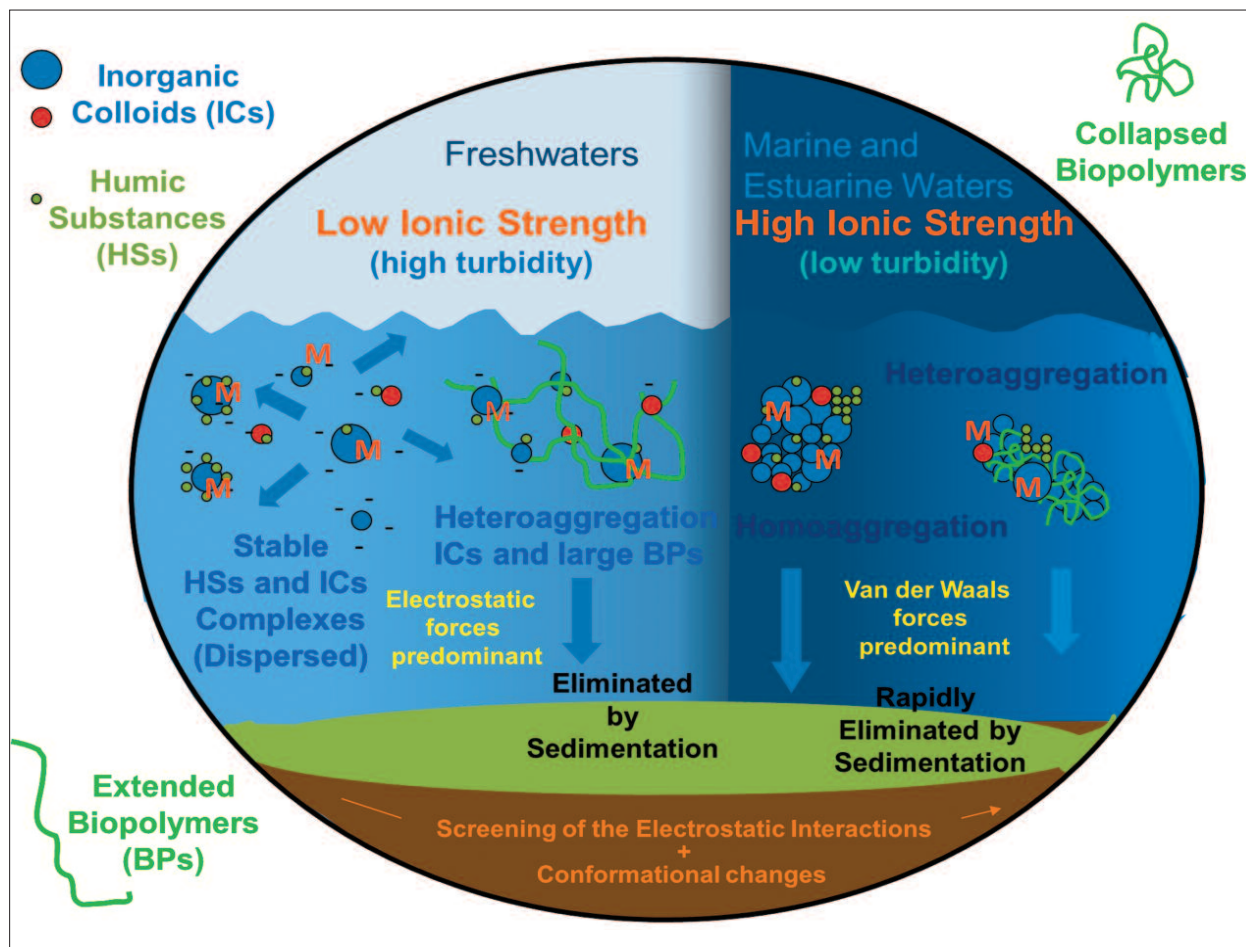
Fig. 4. Major colloidal interactions and aggregation processes relevant in natural waters. At low ionic strength (freshwaters), the electrostatic is expected to play a key role and form stable complexes (high turbidity). Bridging of inorganic colloids by large biopolymers represents the major route for aggregate formation and TM elimination by sedimentation processes. In marine and estuarine waters, due to the increase of the ionic strength and resulting charge screening effects, van der Waals forces are predominant. Homoaggregation as well as heterocoagulation are rapidly promoted resulting in the rapid destabilization, and sedimentation (low turbidity) of the aquatic colloids and thus transport of TMs. Biopolymers are expected to undergo large conformational changes from coils (compact structures) in marine waters to rod-like (extended structures) conformations in freshwaters.
